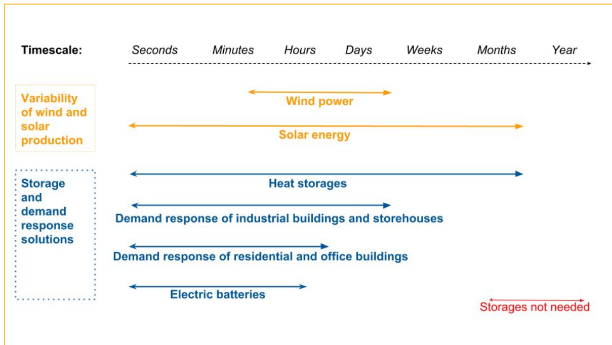
Figure 4: Different storages and demand response solutions offer the flexibility needed because of the variable wind and solar power production
