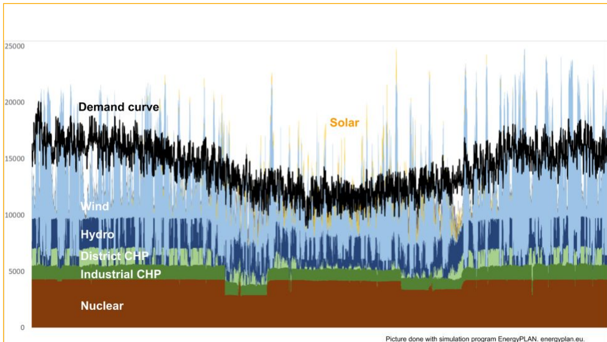
Figure 9. Estimated hourly electricity production in Finland during one year, with a 60 TWh capacity of wind power. Hydro power, combined heat and power (CHP) production in district heating networks and electricity imports are used to even out the power fluctuations. In practice the CHP production curve is smoother than in the picture, due to the e.g. flexible power consumption.
