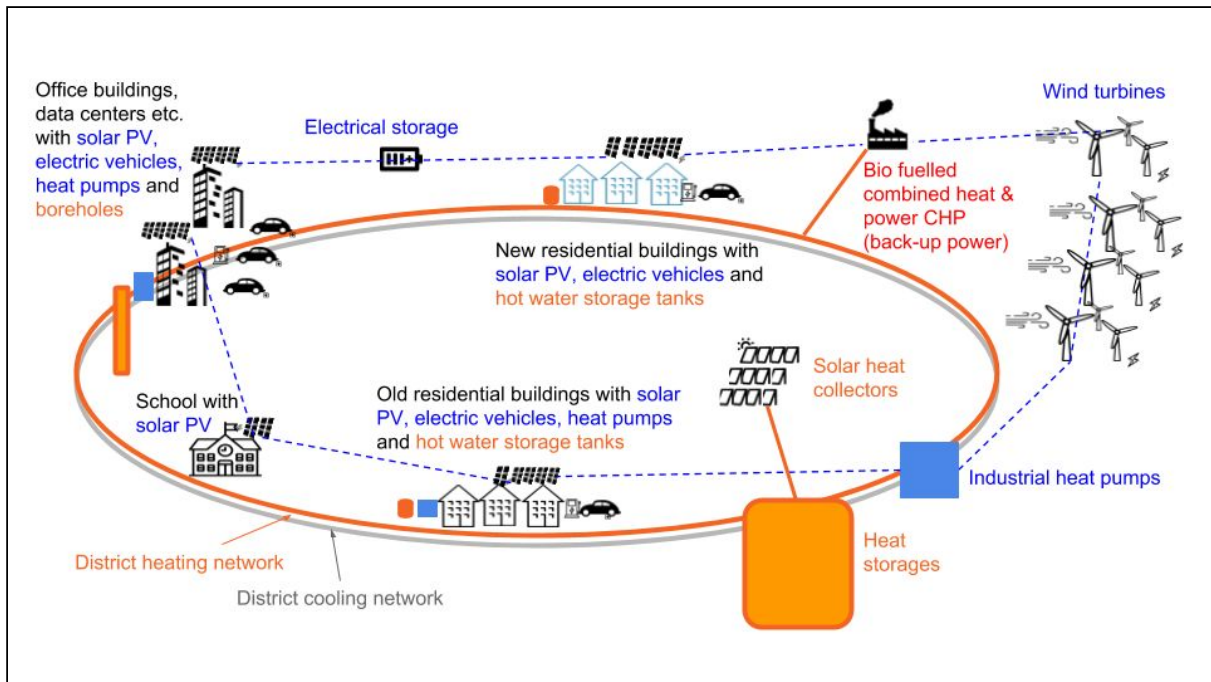
Figure 2: Fossil fuel-free district heating and cooling system
