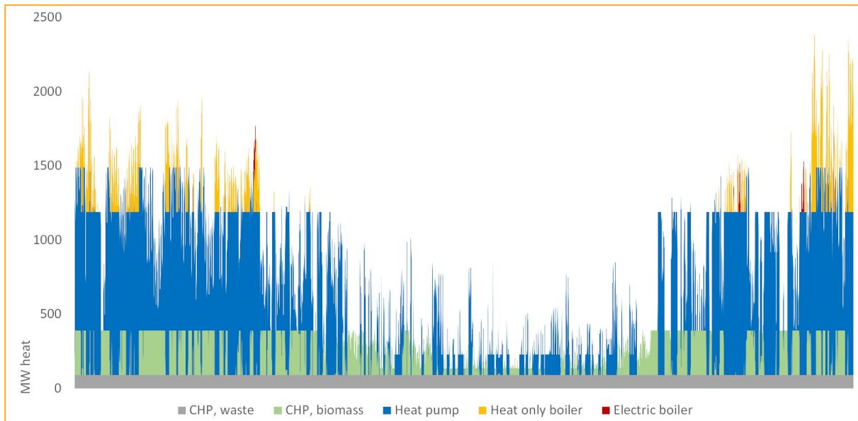
Figure 12. The district heat production in Helsinki hour-by-hour based on 100% fossil-free energy scenario during a year. In reality the running patterns are significantly smoother than in this figure drawn with EnergyPLAN simulation tool.
