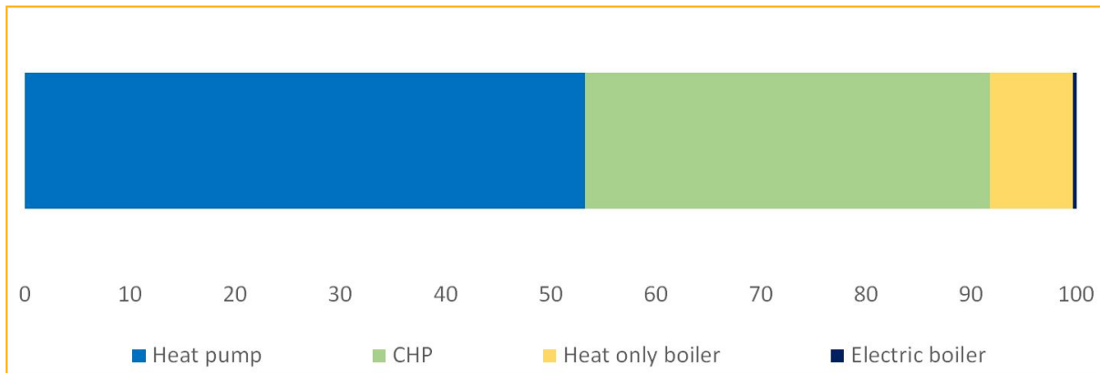
Figure 11. The annual shares of district heating production methods in Finland in the 100 % fossil fuel-free scenario. These shares with combined heat and power (CHP) production concern larger district heating networks, that account for about 75% of the district heating use in Finland.
