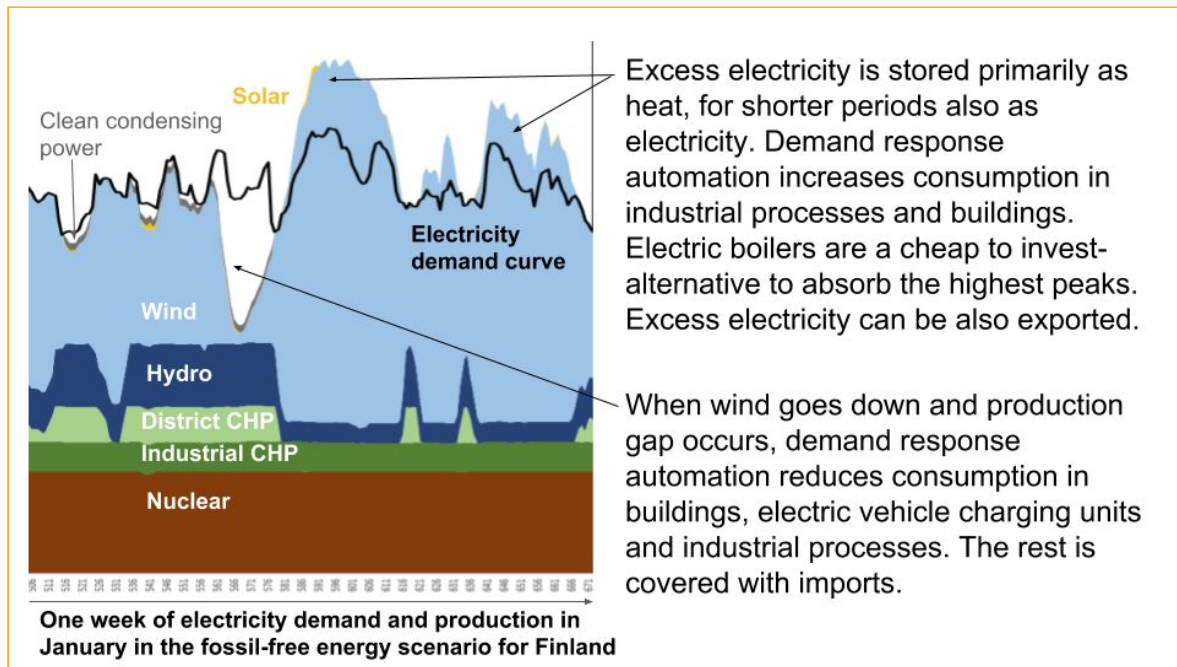
Figure 10. During the coldest days of the year different energy sources, energy storages, demand response solutions, and imports and exports of electricity help to balance the electricity production and demand curves. The amount of imports in the 100% fossil fuel-free scenario is however low, only about third of 2017 year's levels.
