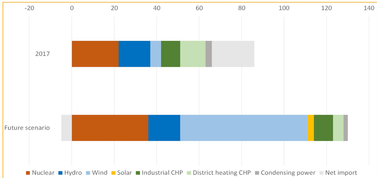
Figure 8. Electricity production in 2017 and in the 100% fossil-free scenario.
